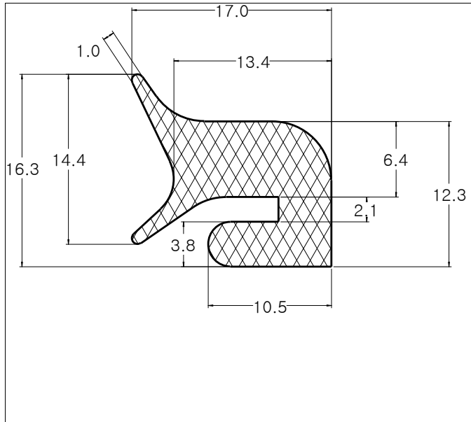
Die No: 8899 Category: Tank-Seal
