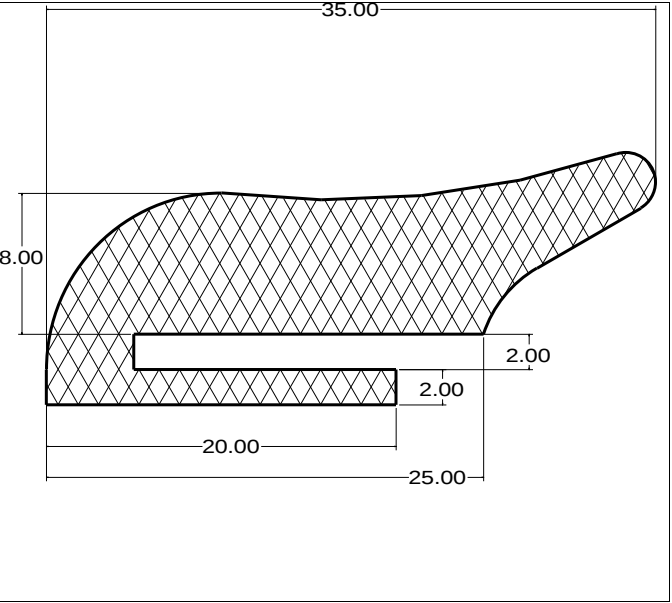
Die No: 5855 Category: Tank-Seal
