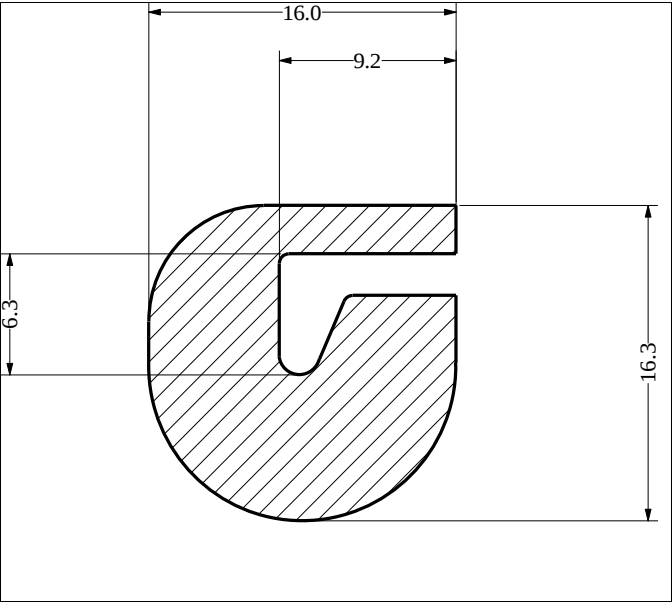
Die No: 2060 Category: Tank-Seal
