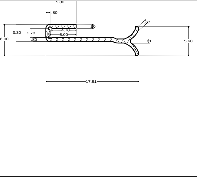
Die No: 4355 Category: Tank-Seal
