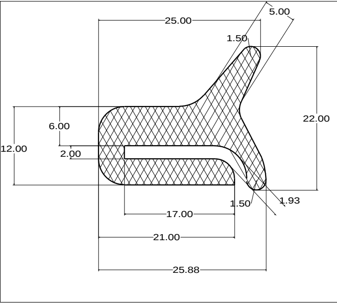
Die No: 4771 Category: Tank-Seal
