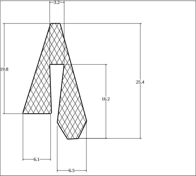
Die No: 4171 Category: Tank-Seal
