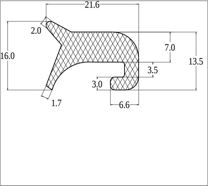
Die No: 9951 Category: Tank-Seal
