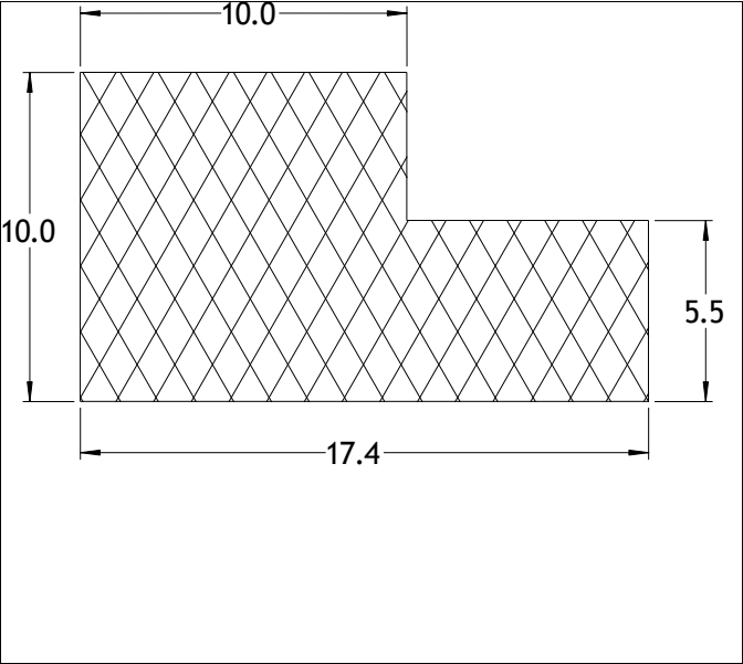
Die No: 6470 Category: L-Section
