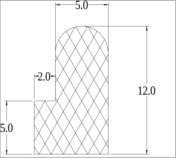
Die No: 9367 Category: L-Section
