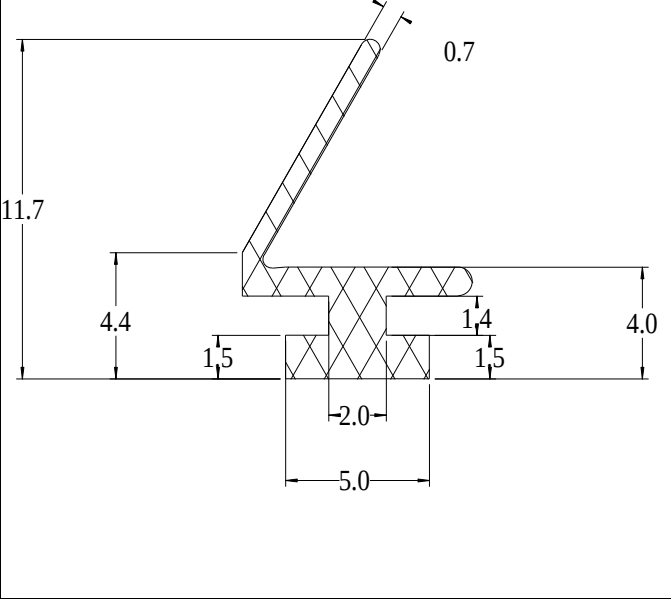
Die No: 9692 Category: L-Section
