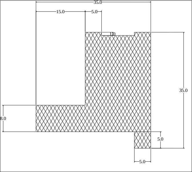
Die No: 3797 Category: L-Section
