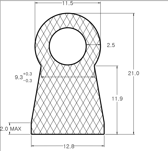
Die No: 8386 Category: Key-Hole
