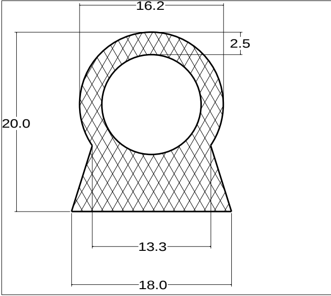
Die No: 4696 Category: Key-Hole
