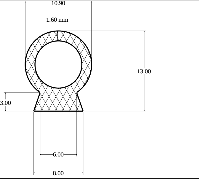
Die No: 3559 Category: Key-Hole
