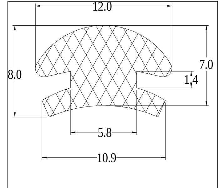
Die No: 9990 Category: H-section
