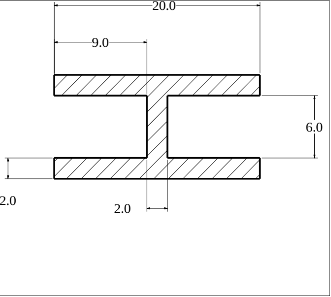
Die No: 1971 Category: H-section
