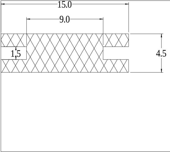
Die No: 9600 Category: H-section
