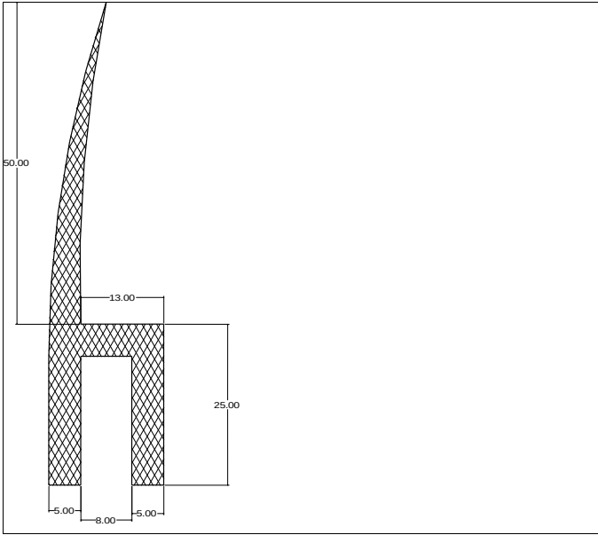
Die No: 4061 Category: H-section
