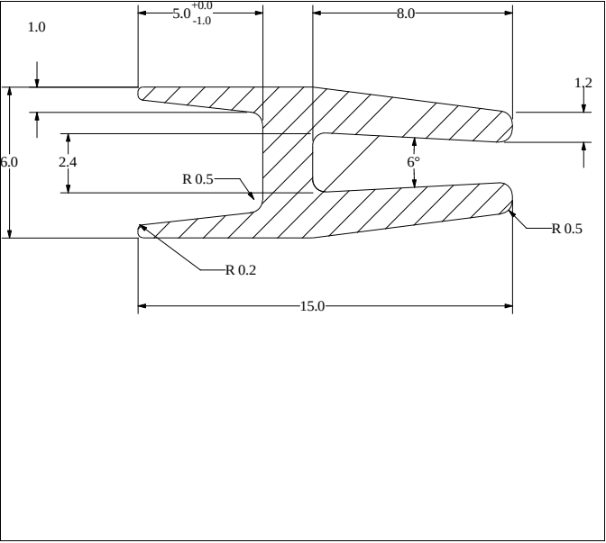
Die No: 1826 Category: H-section
