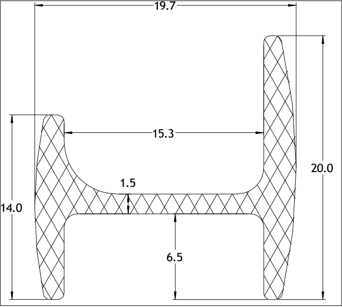
Die No: 7367 Category: H-section
