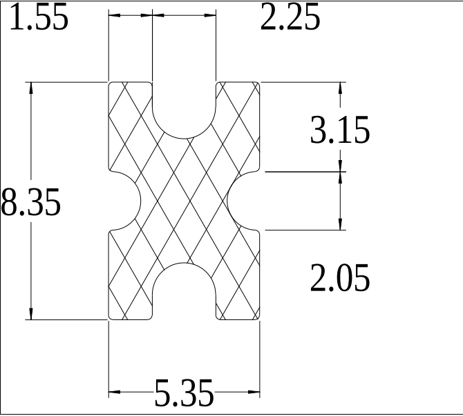
Die No: 9800 Category: H-section
