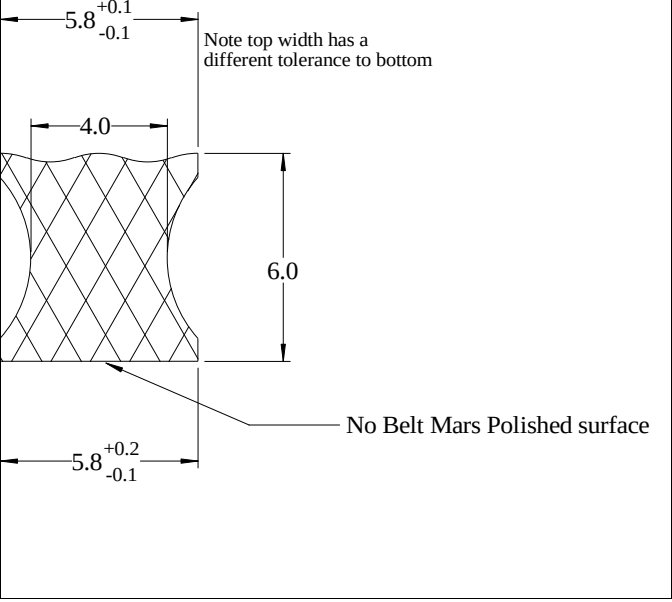
Die No: 5375 Category: H-section
