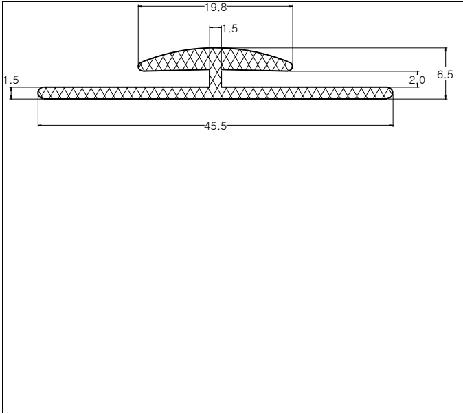
Die No: 9060 Category: H-section
