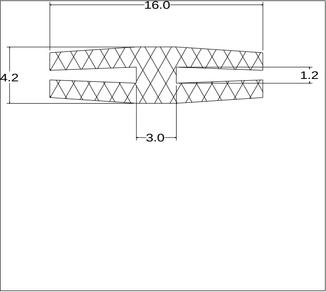
Die No: 4823 Category: H-section
