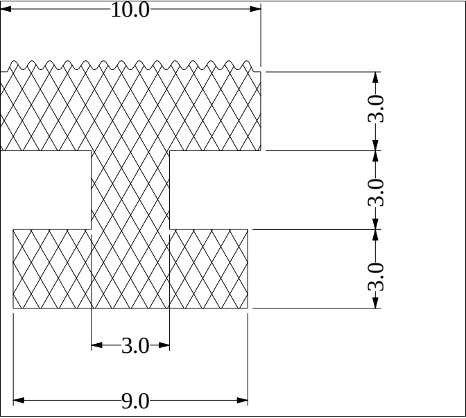
Die No: 1756 Category: H-section
