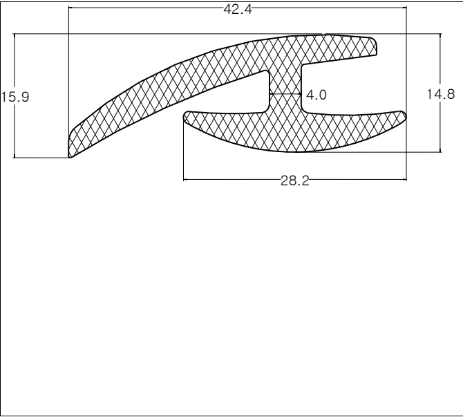
Die No: 9055 Category: H-section
