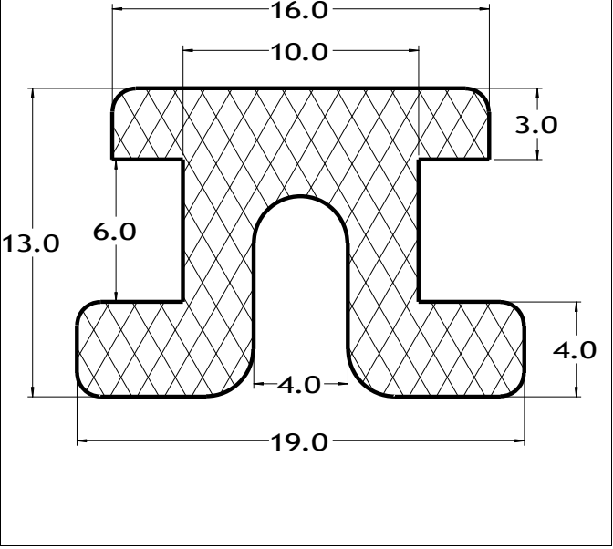
Die No: 7517 Category: H-section
