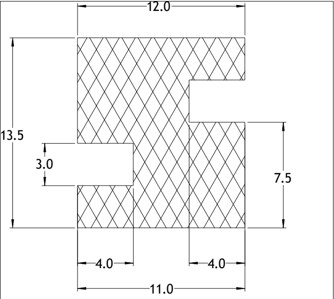
Die No: 6661 Category: H-section
