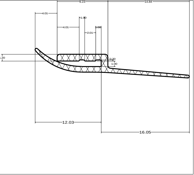
Die No: 4294 Category: H-section
