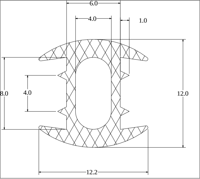
Die No: 3647 Category: H-section
