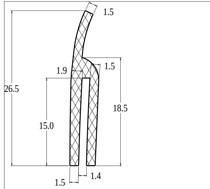
Die No: 9278 Category: H-section
