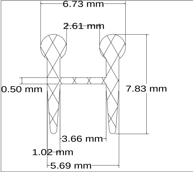
Die No: 3881 Category: H-section
