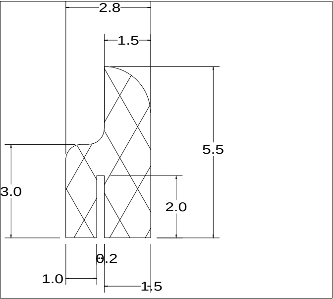
Die No: 5393 Category: H-section
