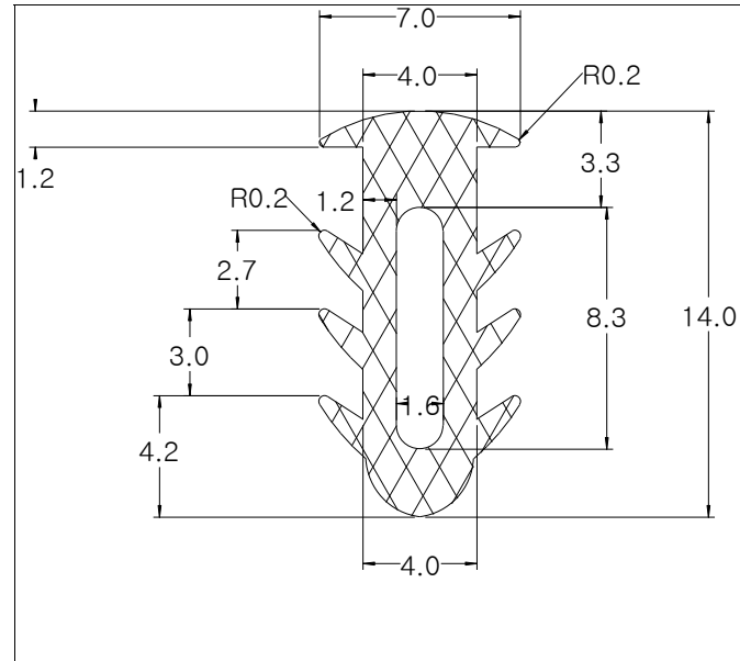
Die No: 8866 Category: T-Section
