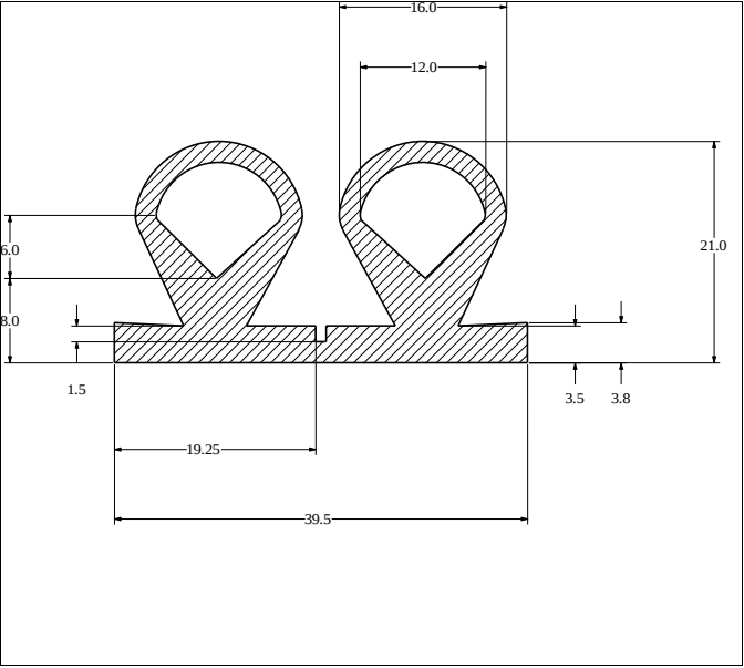
Die No: 1805 Category: P-Double
