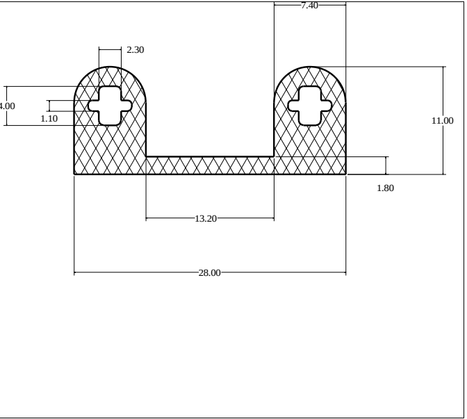
Die No: 3574 Category: P-Double
