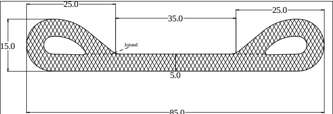
Die No: 5431 Category: P-Double
