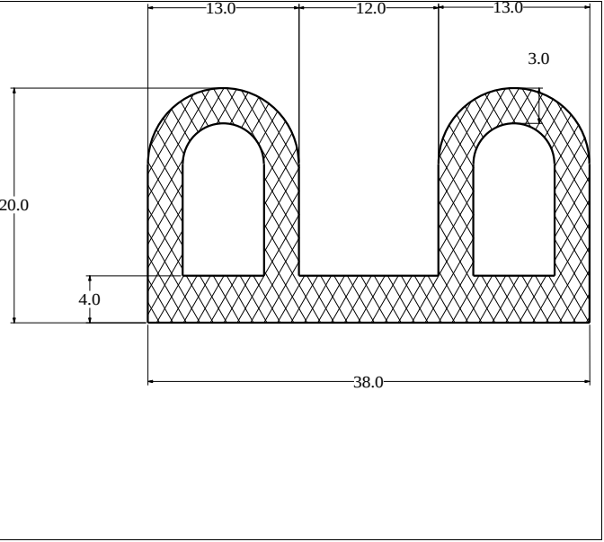
Die No: 2957 Category: P-Double
