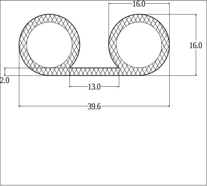
Die No: 5005 Category: P-Double
