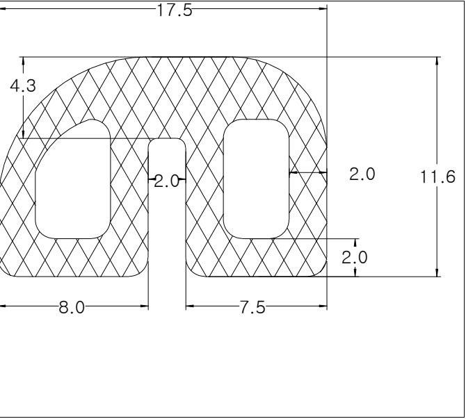
Die No: 7977 Category: P-Double
