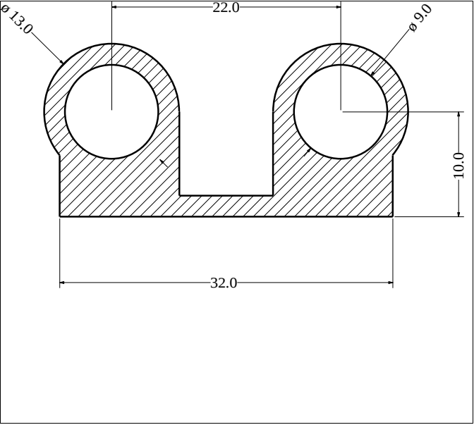
Die No: 465 Category: P-Double
