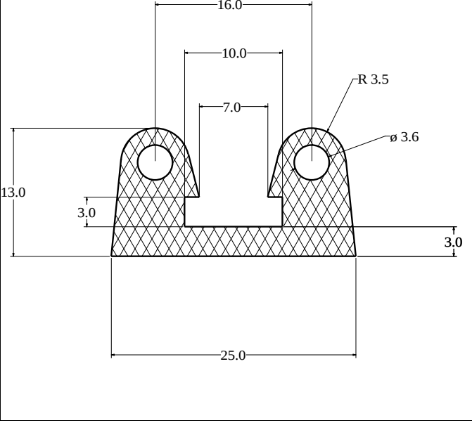
Die No: 2711 Category: P-Double
