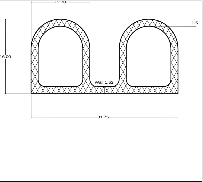
Die No: 5060 Category: P-Double
