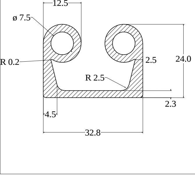
Die No: 2340 Category: P-Double
