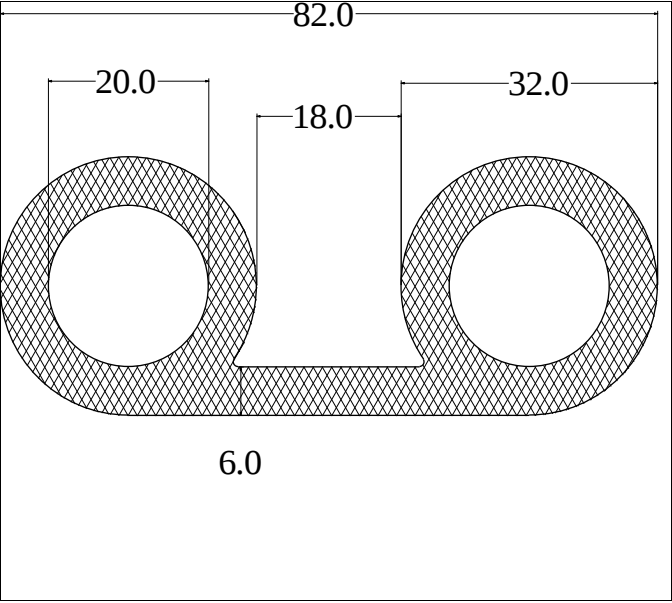
Die No: 2863 Category: P-Double
