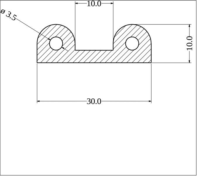
Die No: 429 Category: P-Double
