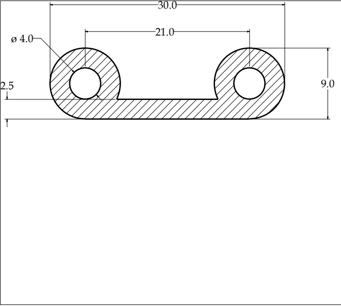
Die No: 1839 Category: P-Double
