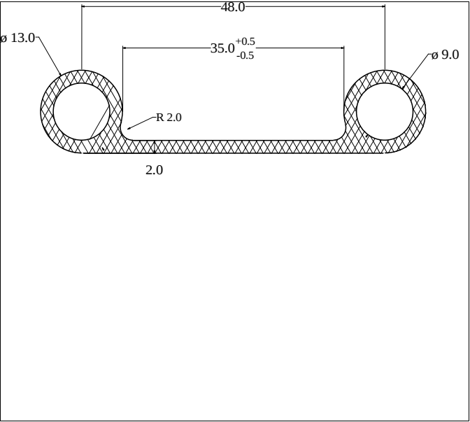
Die No: 2894 Category: P-Double
