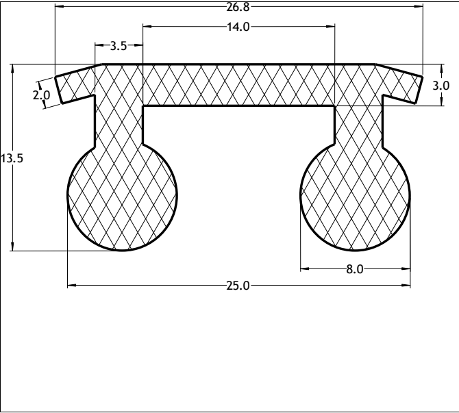
Die No: 7887 Category: P-Double
