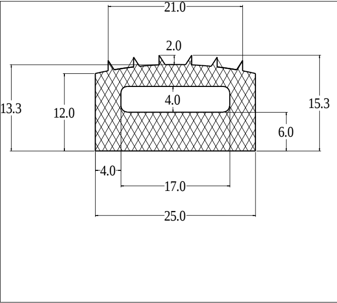
Die No: 9652 Category: Hollow Strip
