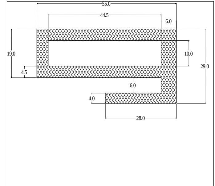
Die No: 9530 Category: E-Section
