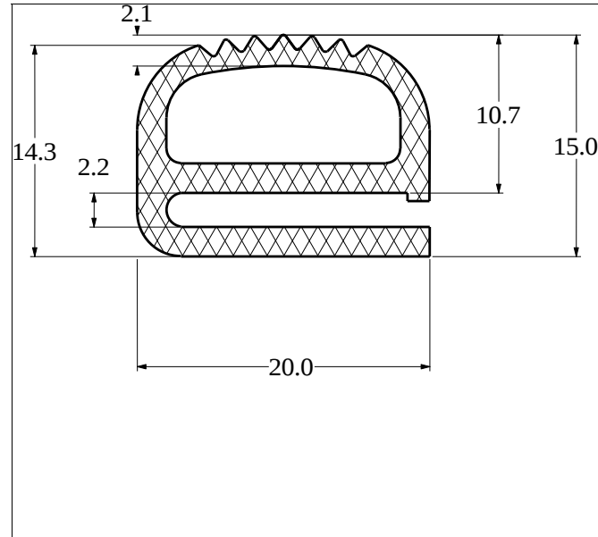
Die No: 3395 Category: E-Section
