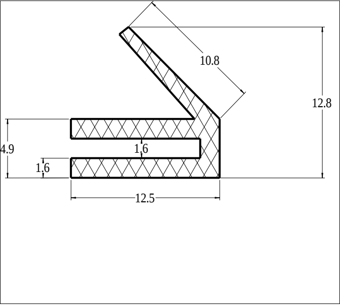
Die No: 9670 Category: E-Section
