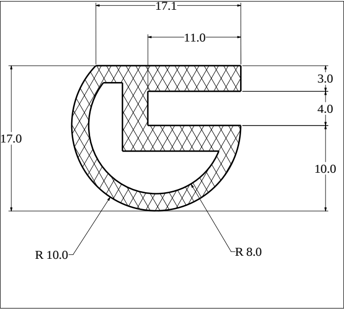
Die No: 2378 Category: E-Section
