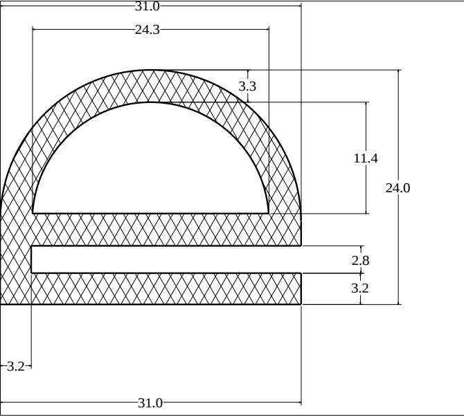
Die No: 3800 Category: E-Section
