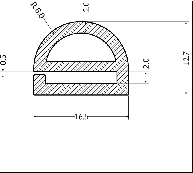
Die No: 1718 Category: E-Section
