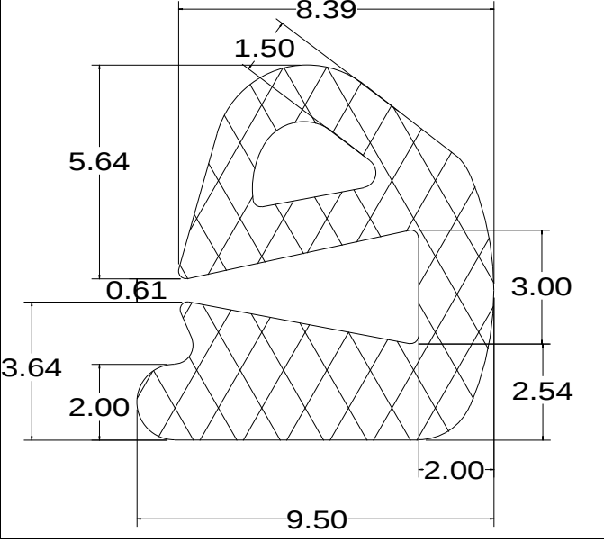
Die No: 4152 Category: E-Section
