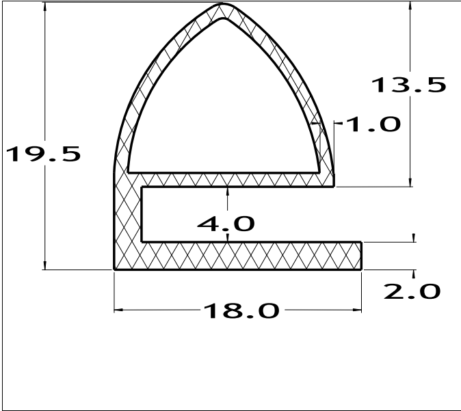
Die No: 7519 Category: E-Section
