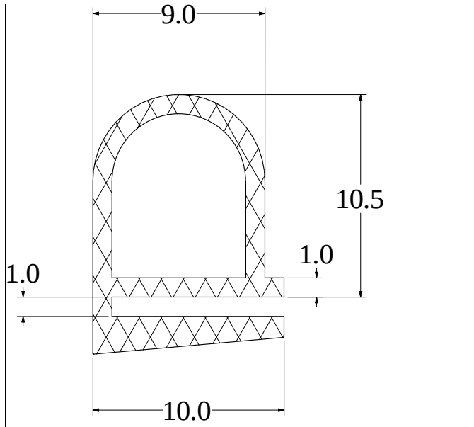
Die No: 2437 Category: E-Section
