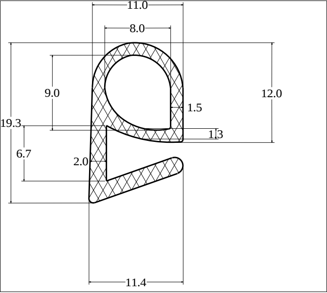
Die No: 3793 Category: E-Section
