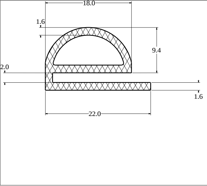
Die No: 2271 Category: E-Section
