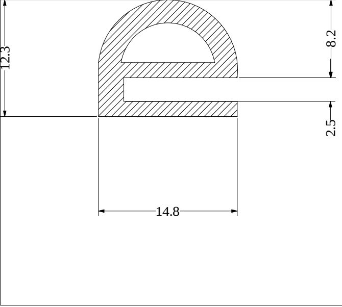
Die No: 644 Category: E-Section
