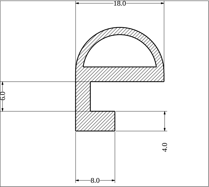
Die No: 1055 Category: E-Section
