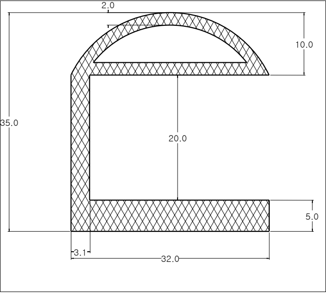
Die No: 8753 Category: E-Section
