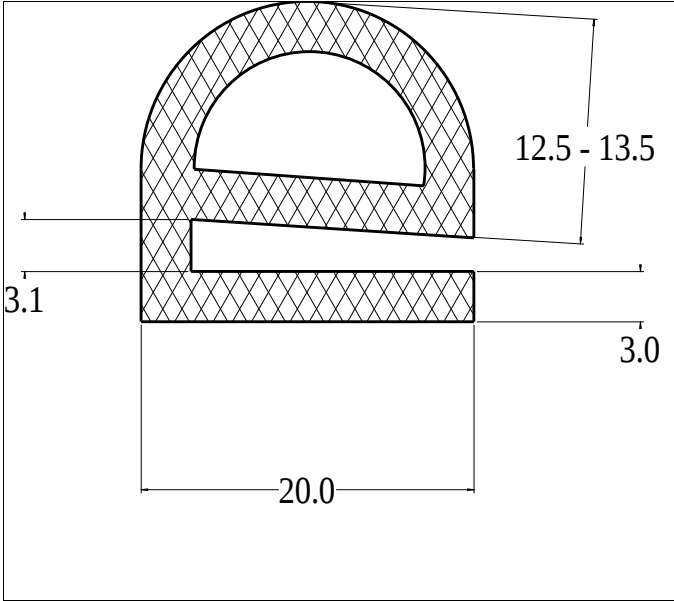
Die No: 1180 Category: E-Section
