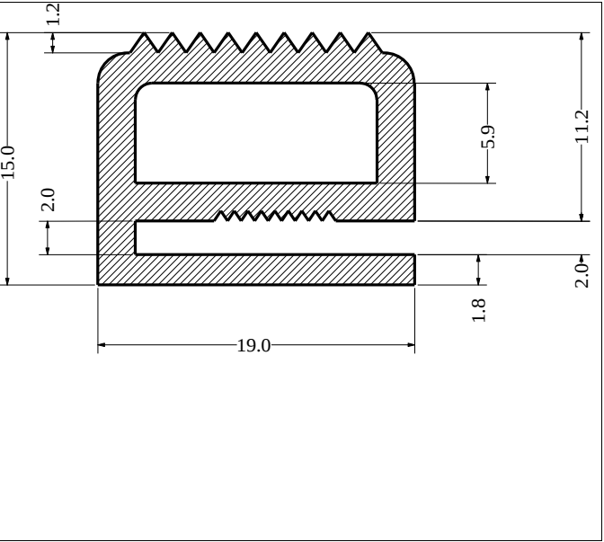
Die No: 1727 Category: E-Section
