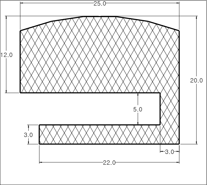
Die No: 8650 Category: E-Section
