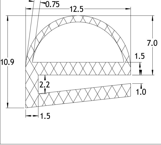
Die No: 6102 Category: E-Section
