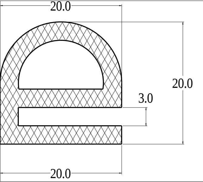
Die No: 9078 Category: E-Section
