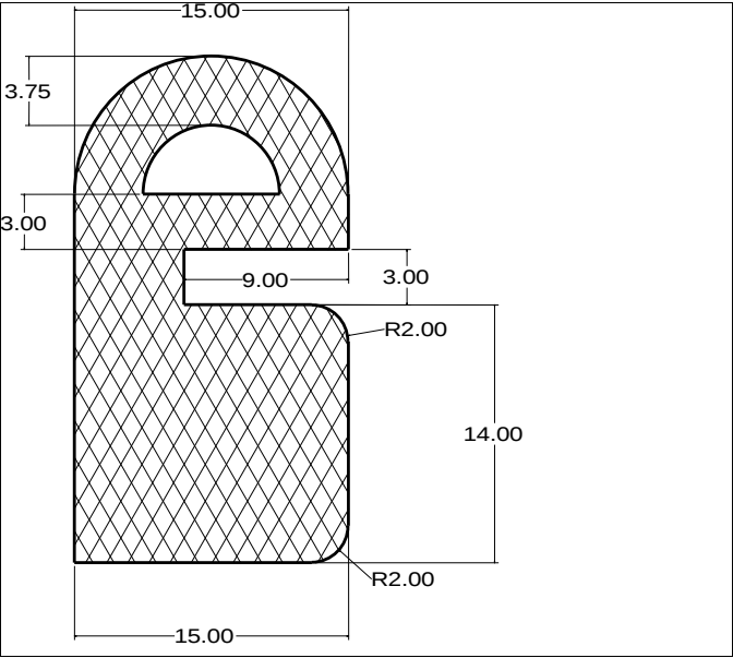
Die No: 8353 Category: E-Section
