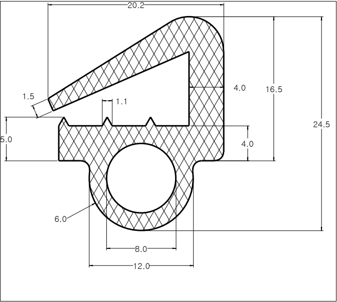
Die No: 8805 Category: E-Section
