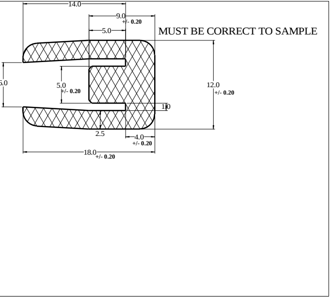
Die No: 5496 Category: E-Section
