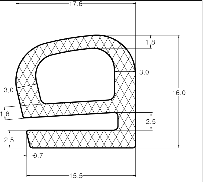
Die No: 8687 Category: E-Section
