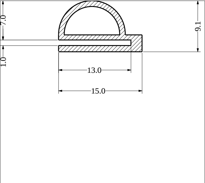
Die No: 6244 Category: E-Section
