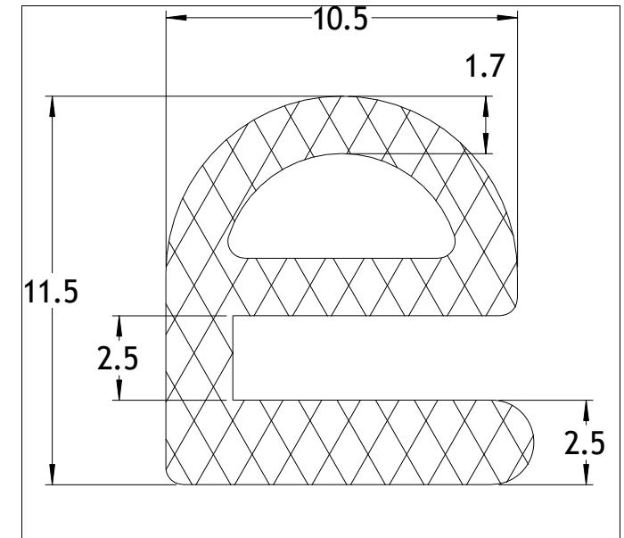
Die No: 7301 Category: E-Section
