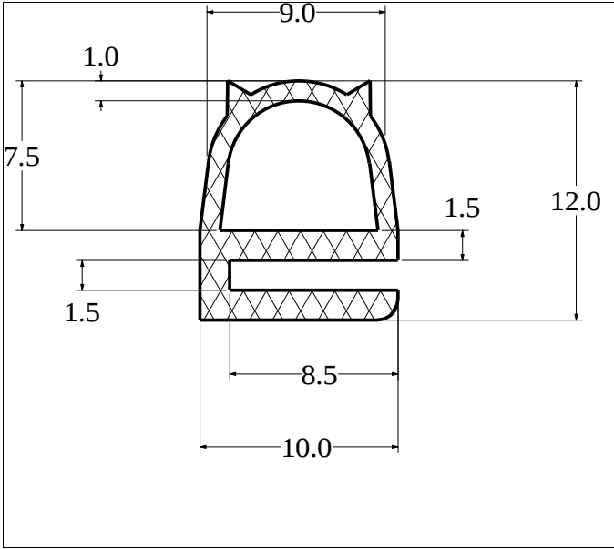
Die No: 2411 Category: E-Section
