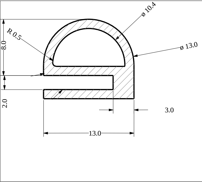
Die No: 1436 Category: E-Section
