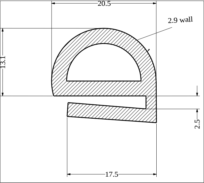
Die No: 4444 Category: E-Section
