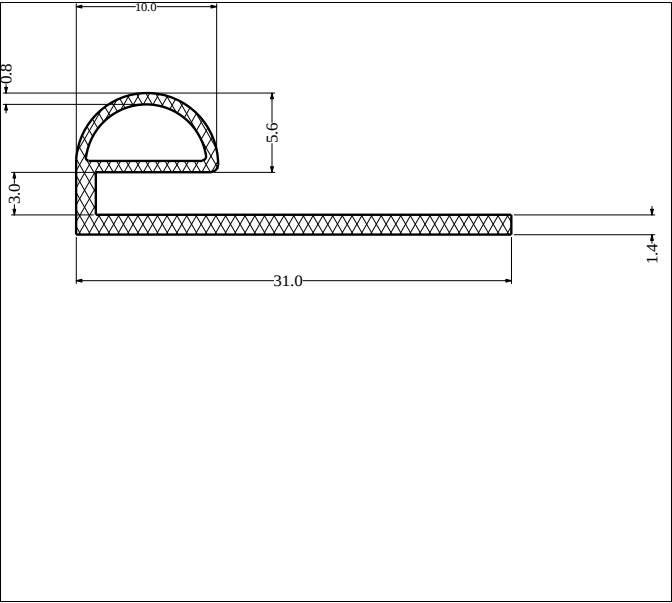
Die No: 1850 Category: E-Section
