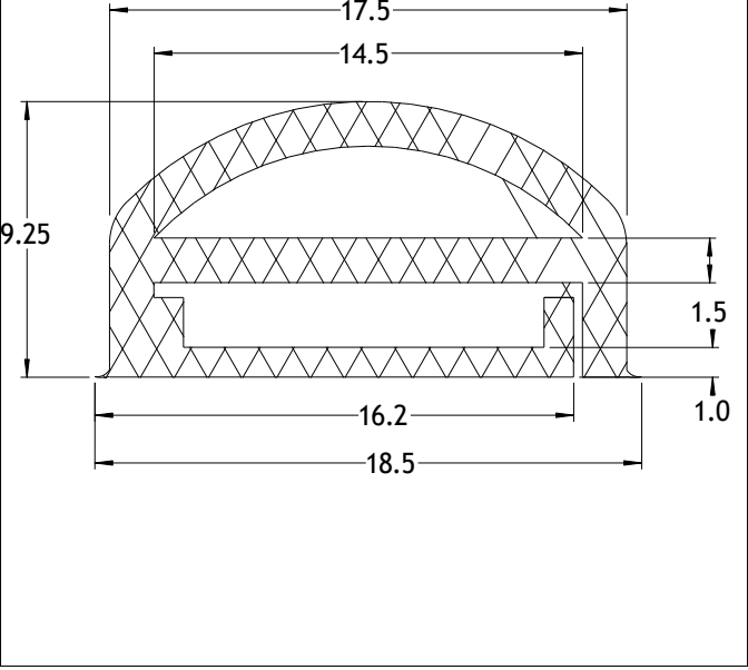
Die No: 6057 Category: E-Section
