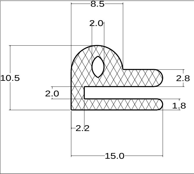
Die No: 4937 Category: E-Section
