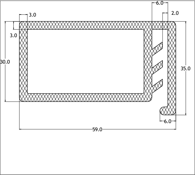
Die No: 7050 Category: E-Section
