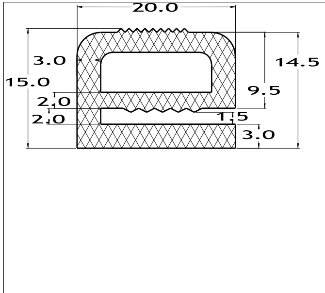
Die No: 7575 Category: E-Section
