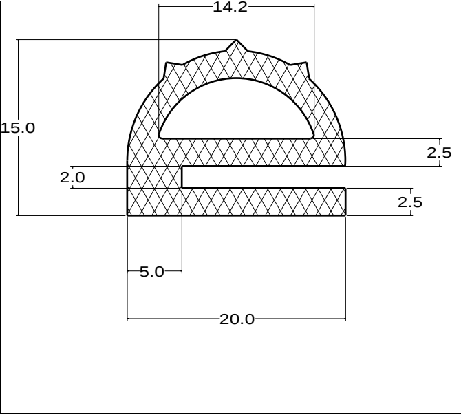
Die No: 4670 Category: E-Section
