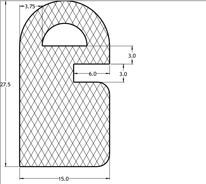
Die No: 6848 Category: E-Section
