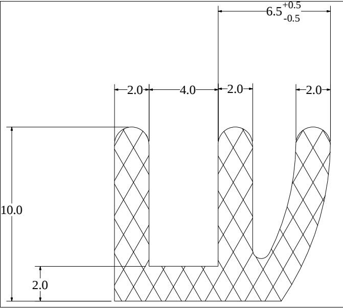
Die No: 3701 Category: E-Section
