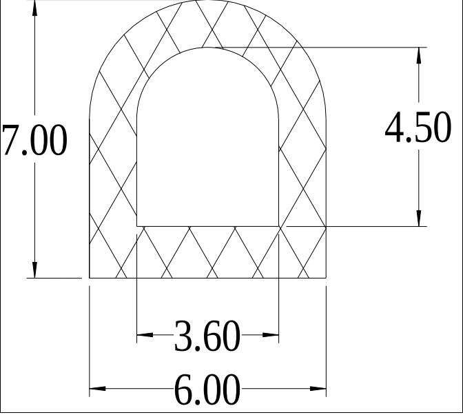
Die No: 9786 Category: D-Hollow
